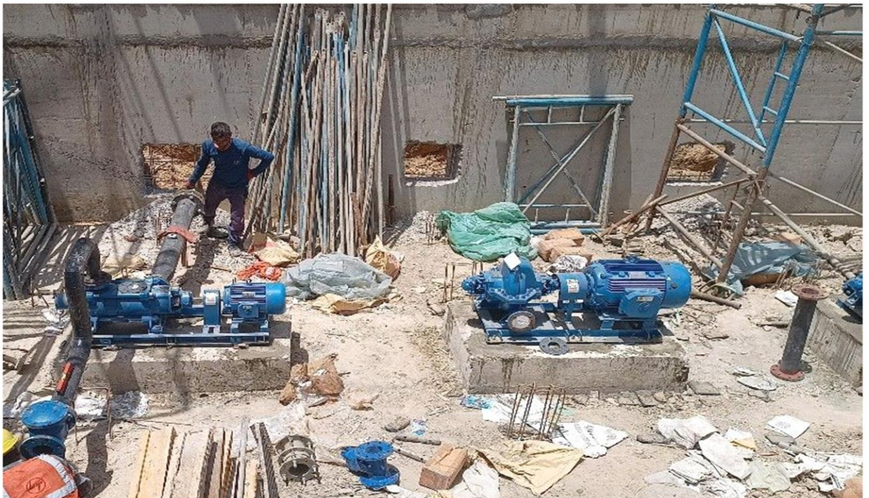
Pump House Construction with Industrial Shade
